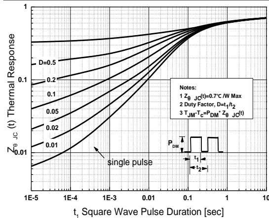
Transient Thermal Response Curve For AJCS10N65CT
